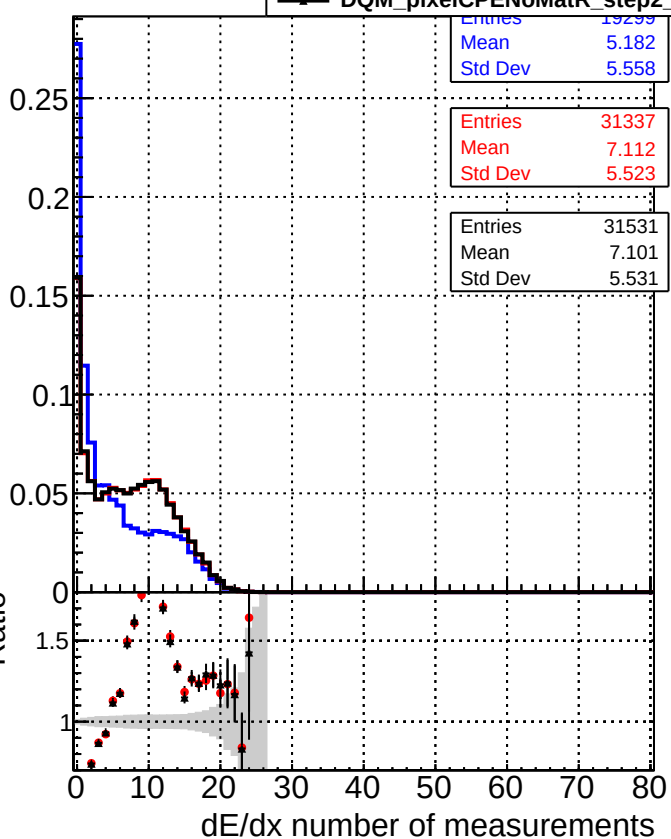
— DQM_original_step2_ttbar-phase1-newgeom — DQM_pixelCPE_step2_ttbar-phase1-newgeom — DQM_pixelCPENoMatR_step2_ttbar-phase1-newgeom
