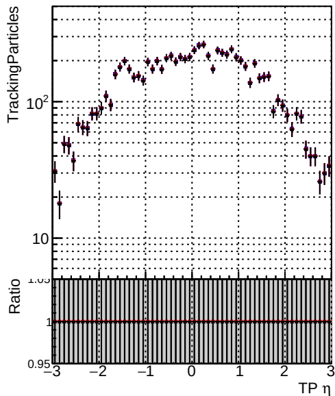
—•— DQM_original_step2_ttbar-phase1-newgeom —•— DQM_pixelCPE_step2_ttbar-phase1-newgeom —•— DQM_pixelCPENoMatR_step2_ttbar-phase1-newgeom
