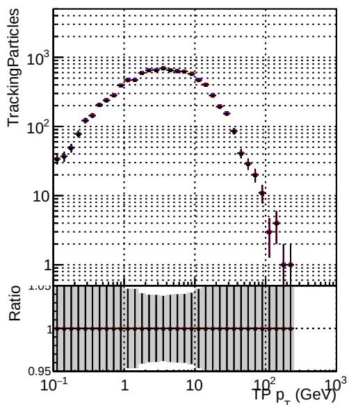
—•— DQM_original_step2_ttbar-phase1-newgeom —•— DQM_pixelCPE_step2_ttbar-phase1-newgeom —•— DQM_pixelCPENoMatR_step2_ttbar-phase1-newgeom
