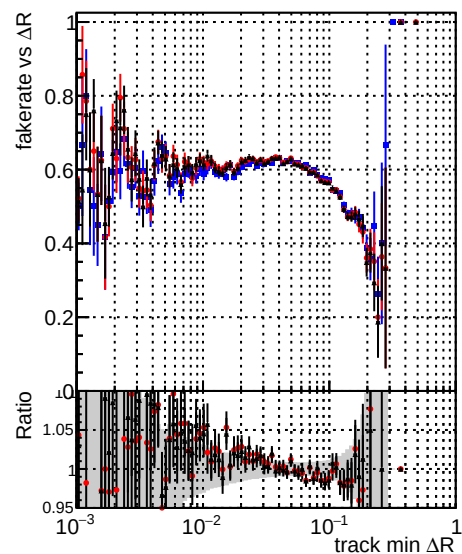
— DQM original step2 ttbar-phase1-newgeom — DQM pixelCPE step2 ttbar-phase1-newgeom — DQM pixelCPENoMatR step2 ttbar-phase1-newgeom
