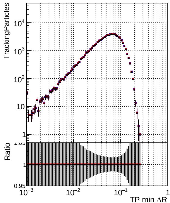
N of simulated tracks ■ DQM_original_step2_ttbar-phase1-newgeom ● DQM_pixelCPE_step2_ttbar-phase1-newgeom ▲ DQM_pixelCPEChi2OR_step2_ttbar-phase1-newgeom
