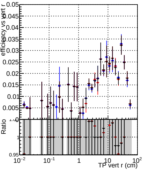
Efficiency vs vertpos DQM_original_step2_ttbar-phase1-newgeom DQM_pixelCPE_step2_ttbar-phase1-newgeom DQM_pixelCPEChi2OR_step2_ttbar-phase1-newgeom
