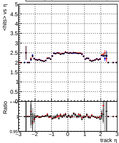
mean hits — DQM_original_step2_ttbar-phase1-newgeom — DQM_pixelCPE_step2_ttbar-phase1-newgeom — DQM_pixelCPEChi2OR_step2_ttbar-phase1-newgeom
