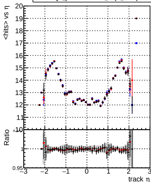
mean hits vs \eta — DQM_original_step2_ttbar-phase1-newgeom — DQM_pixelCPE_step2_ttbar-phase1-newgeom — DQM_pixelCPEChi2OR_step2_ttbar-phase1-newgeom
