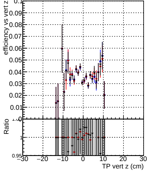
Efficiency vs. sim PV z —●— DQM_original_step2_ttbar-phase1-newgeom —●— DQM_pixelCPE_step2_ttbar-phase1-newgeom —●— DQM_pixelCPEChi2OR_step2_ttbar-phase1-newgeom
