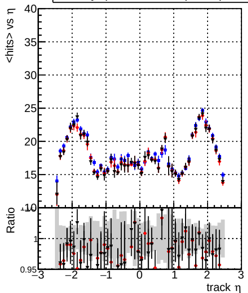
— DQM_original_step2_ttbar-phase1-newgeom — DQM_pixelCPE_step2_ttbar-phase1-newgeom — DQM_pixelCPEChi2OR_step2_ttbar-phase1-newgeom mean hits
