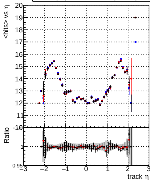
mean hits — DQM_original_step2_ttbar-phase1-newgeom — DQM_pixelCPE_step2_ttbar-phase1-newgeom — DQM_pixelCPEChi2OR_step2_ttbar-phase1-newgeom
