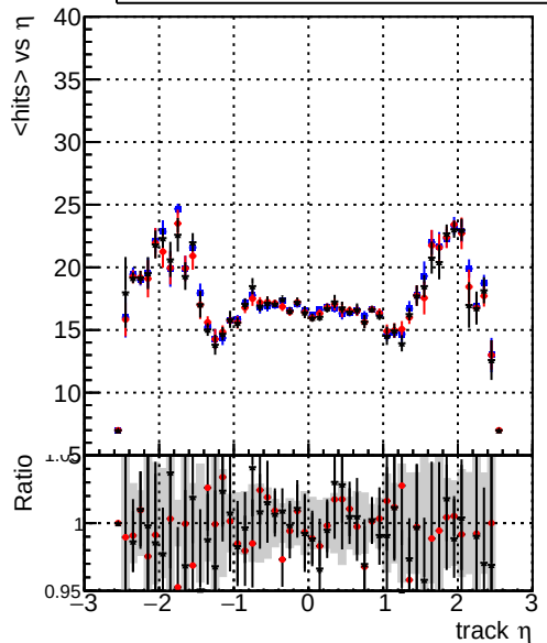
mean hits — DQM_original_step2_ttbar-phase1-newgeom — DQM_pixelCPE_step2_ttbar-phase1-newgeom — DQM_pixelCPEChi2OR_step2_ttbar-phase1-newgeom
