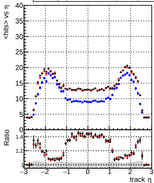
— DQM_original_step2_ttbar-phase1-newgeom — DQM_pixelCPE_step2_ttbar-phase1-newgeom — DQM_pixelCPEChi2OR_step2_ttbar-phase1-newgeom mean hits
