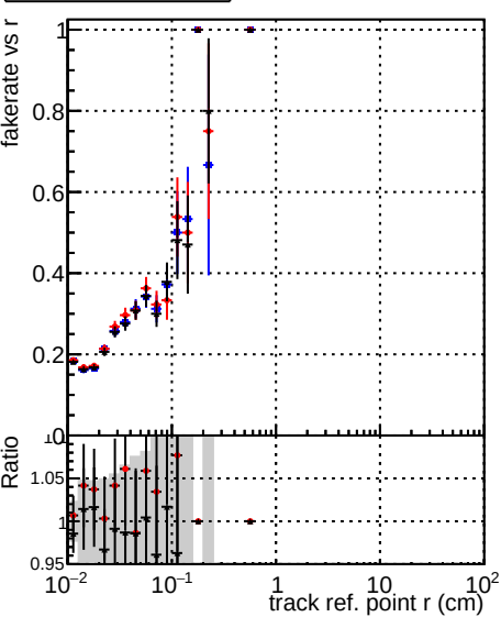
Fake rate vs verpos — DQM_original_step2_ttbar-phase1-newgeom — DQM_pixelCPE_step2_ttbar-phase1-newgeom — DQM_pixelCPEChi2OR_step2_ttbar-phase1-newgeom
