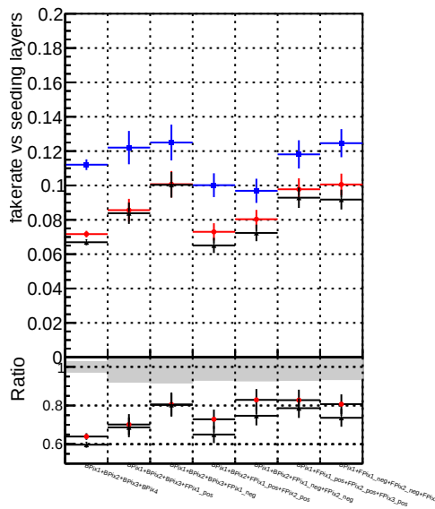
Fake rate vs. — DOM original step2 ttbar-phase1-newgeom — step2 ttbar-phase1-newgeom — DOM pixelCPEch2OR step2 ttbar-phase1-newgeom
