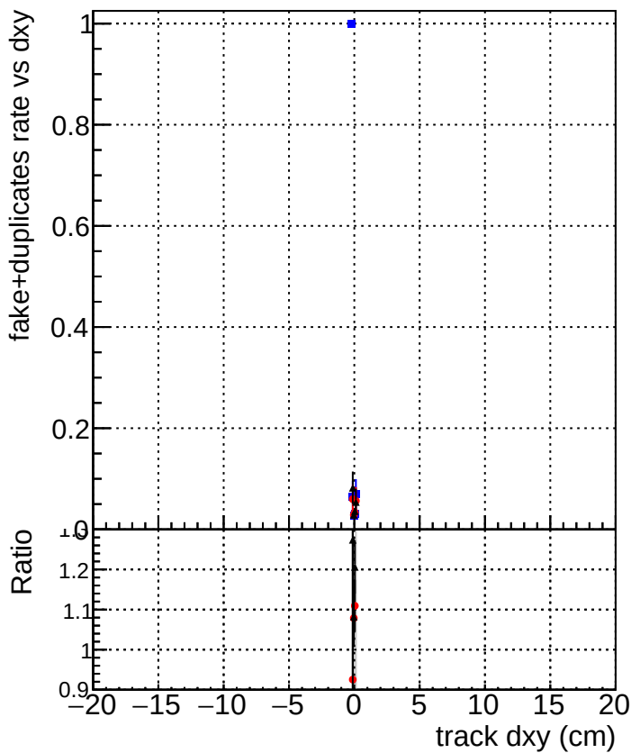
Legend for the bottom plot: ■ DQM_original_step2_ttbar-phase1-newgeom ● DQM_pixelCPE_step2_ttbar-phase1-newgeom ▲ DQM_pixelCPEChi2OR_step2_ttbar-phase1-newgeom
