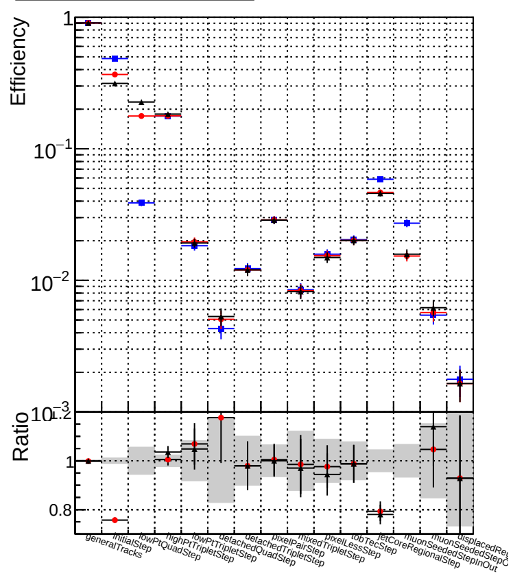
DQM_original_step2_ttbar-phase1-newgeom DQM_pixelCPE_step2_ttbar-phase1-newgeom DQM_pixelCPEChi2OR_step2_ttbar-phase1-newgeom
