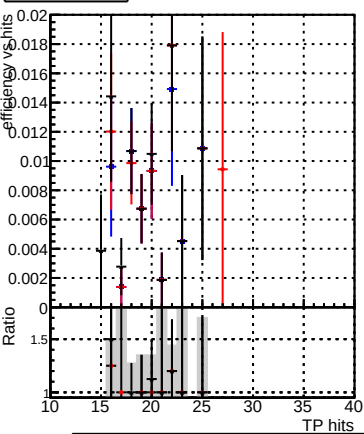
Efficiency vs hit Legend: DQM_original_step2_ttbar-phase1-newgeom DQM_pixelCPE_step2_ttbar-phase1-newgeom DQM_pixelCPEChi2OR_step2_ttbar-phase1-newgeom
