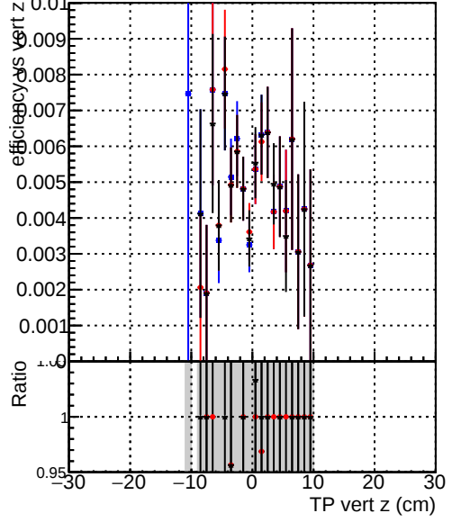
Efficiency vs. TP vert z (cm) — DQM_original_step2_ttbar-phase1-newgeom — DQM_pixelCPE_step2_ttbar-phase1-newgeom — DQM_pixelCPEChi2OR_step2_ttbar-phase1-newgeom
