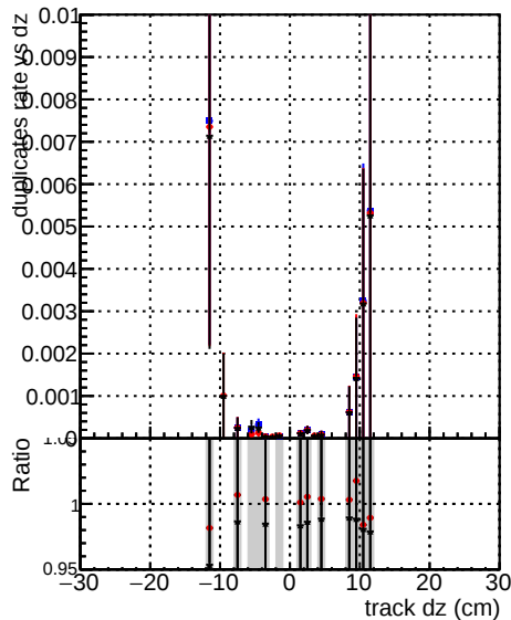
base1-newgeom tbar-phase1-newgeom
