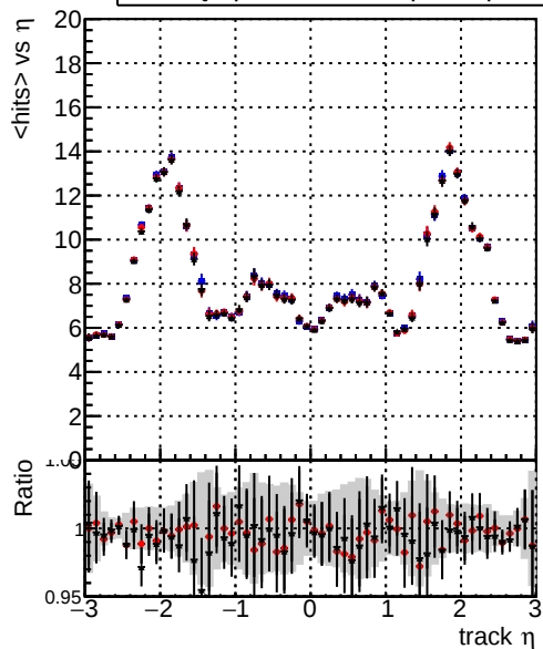
mean hits vs \eta — DQM_original_step2_ttbar-phase1-newgeom — DQM_pixelCPE_step2_ttbar-phase1-newgeom — DQM_pixelCPEChi2OR_step2_ttbar-phase1-newgeom
