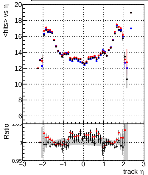
mean hits vs \eta — DQM_original_step2_ttbbar-phase1-newgeom — DQM_pixelCPE_step2_ttbbar-phase1-newgeom — DQM_pixelCPEChi2OR_step2_ttbbar-phase1-newgeom
