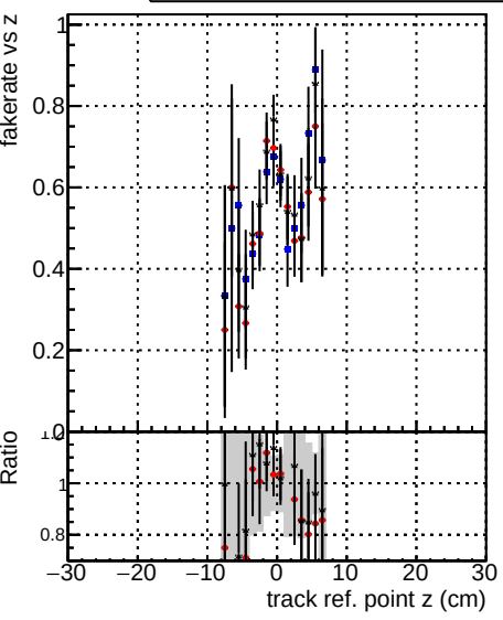
Fake rate vs verpos Legend: DQMstep3_ZToEE_CKF (blue dots) DQMstep3_ZToEE_default (red dots) DQMstep3_ZToEE_ckfPixelLess (black dots)
