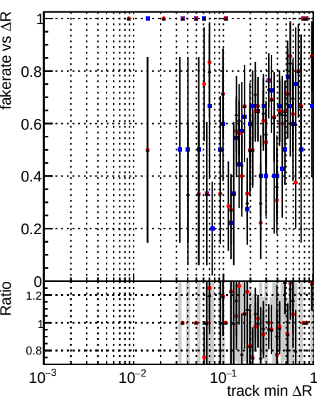
Fake rate vs \Delta R(\text{track, jet}) Legend: DQMstep3_ZToEE_CKF (blue dots) DQMstep3_ZToEE_default (red dots) DQMstep3_ZToEE_ckfPixelLess (black line)
