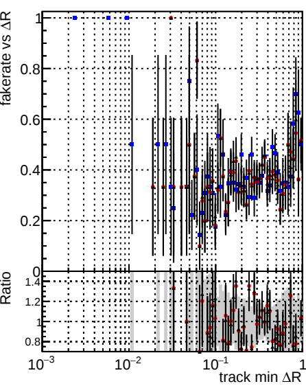
Fake rate vs \Delta R(\text{track, jet}) Legend: DQMstep3_ZToEE_CKF (blue dots) DQMstep3_ZToEE_default (red dots) DQMstep3_ZToEE_ckfPixelLess (black dots)
