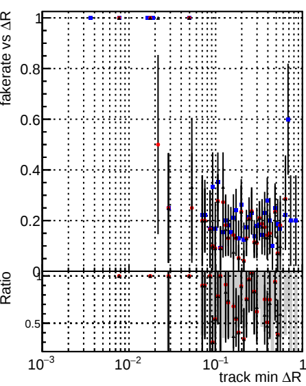
Fake rate vs \Delta R(\text{track, jet}) Legend: DQMstep3_ZToEE_CKF (blue dots) DQMstep3_ZToEE_default (red dots) DQMstep3_ZToEE_ckfPixelLess (black dots with error bars)
