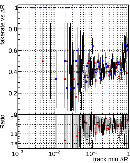
Fake rate vs \Delta R(\text{track, jet}) Legend: DOMstep3_ZToEE_CKF (blue dots) DOMstep3_ZToEE_default (red dots) DOMstep3_ZToEE_ckfPixelLess (black line)
