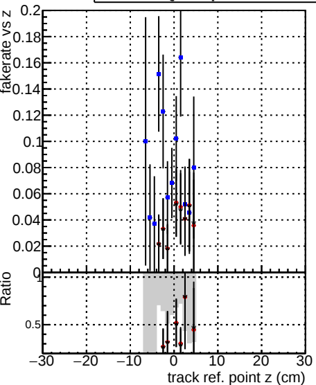
Fake rate vs v —•— DOMstep3_ZToEE_CKF —•— DOMstep3_ZToEE_default —•— DOMstep3_ZToEE_ckfPixelLess
