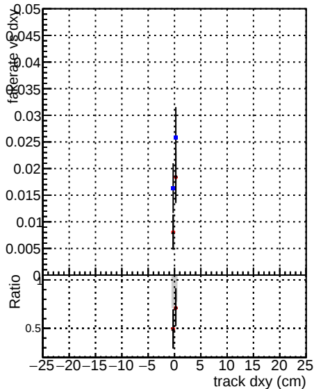
Fake rate vs d DOMstep3 ZToEE CKF DOMstep3 ZToEE default DOMstep3 ZToEE CKFPixelLess
