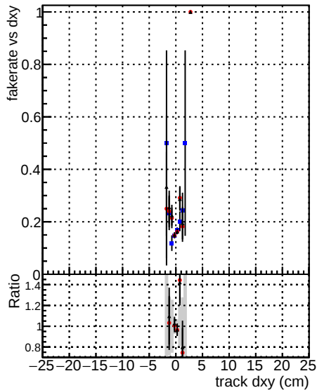
DOMstep3 ZToEE CKF DOMstep3 ZToEE dTight DOMstep3 ZToEE CKFPixelLess
