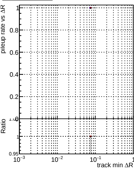
Legend: - DOMstep3_ZToEE_CKF (grey bar) - DOMstep3_ZToEE_default (red dot) - DOMstep3_ZToEE_ckfPixelLess (black line)
