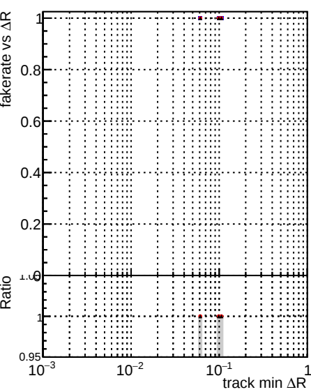
Fake rate vs ΔR(track, jet) Legend: - DQMstep3_ZToEE_CKF (grey line) - DQMstep3_ZToEE_default (red line) - DQMstep3_ZToEE_ckfPixelLess (black line)
