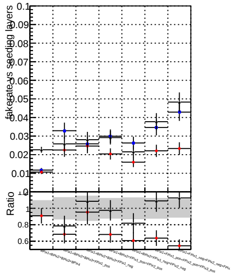
Fake rate vs. DOMstep3 ZToEE CKF DOMstep3 ZToEE default DOMstep3 ZToEE defaultNEWT
