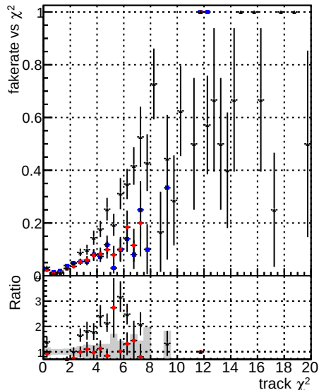
Fake rate vs. DOMstep3 ZToEE CKF DOMstep3 ZToEE default DOMstep3 ZToEE defaultNEWT
