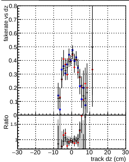
Fake rate vs dz Legend: DOMstep3 ZToEE CKF (blue squares) DOMstep3 ZToEE default (red circles) DOMstep3 ZToEE default NEWT (black circles)
