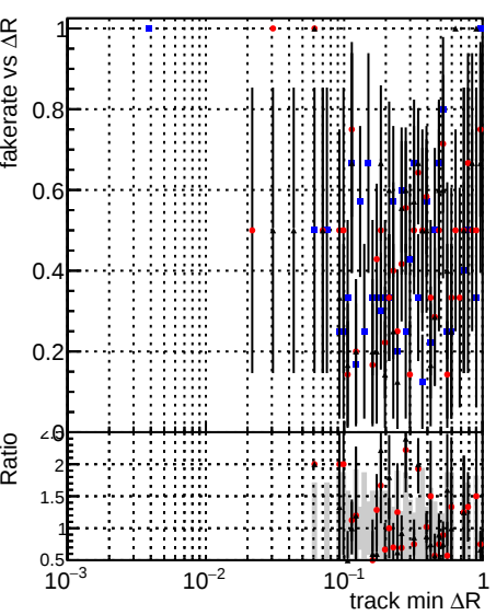
Legend: DQMstep3_ZToEE_CKF (blue dots), DQMstep3_ZToEE_default (red dots), DQMstep3_ZToEE_defaultNEWT (black line with error bars)
