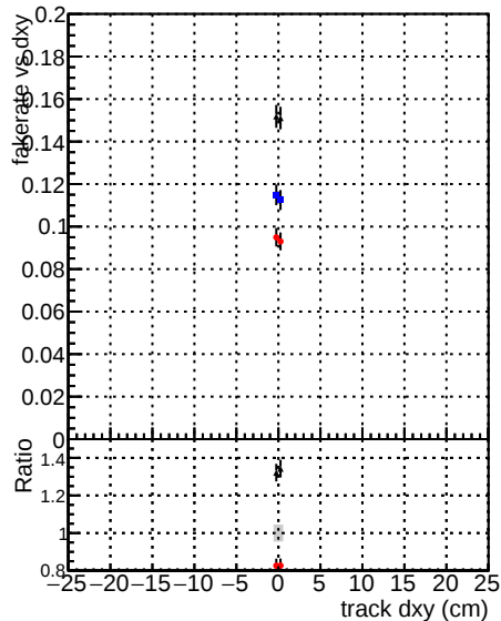
Legend for Fake rate vs dxy, Duplicates Rate vs Dxy, and Pileup rate vs dxy: DOMstep3 ZToEE CKF (blue line) DOMstep3 ZToEE default (red line) DOMstep3 ZToEE default NEWT (grey line)
