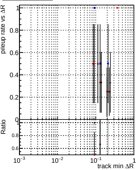
Legend: DOMstep3_ZToEE_CKF (blue dots), DOMstep3_ZToEE_default (red dots), DOMstep3_ZToEE_defaultNEWT (black dots)
