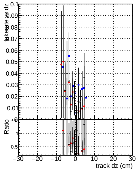
Fake rate vs dz —●— DOMstep3 ZToEE CKF —●— DOMstep3 ZToEE default —●— DOMstep3 ZToEE defaultNEWT
