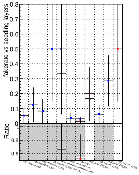
Fake rate vs. DOMstep3 ZToEE CKF DOMstep3 ZToEE default DOMstep3 ZToEE defaultNEWT
