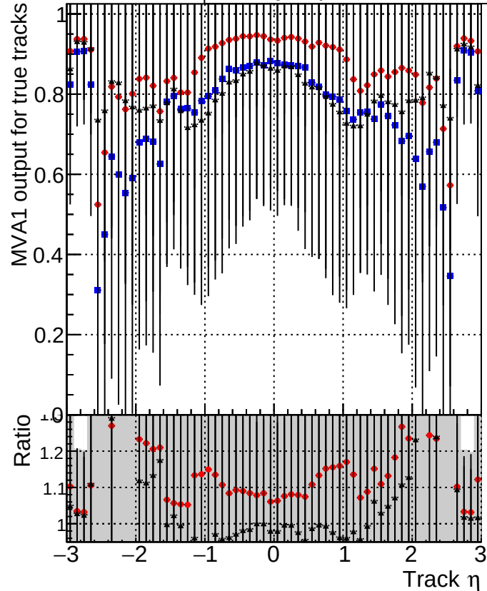
MVA1 of associated tracks (recoToSim) vs. track \eta Legend: DQMstep3_ZToEE_CKF (blue squares) DQMstep3_ZToEE_default (red circles) DQMstep3_ZToEE_defaultNEWT (black stars)
