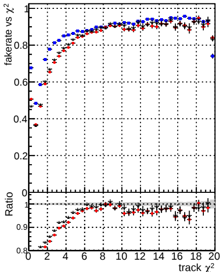
Fake rate vs. DOMstep3 ZToFF CKF DOMstep3 ZToFF default DOMstep3 ZToFF defaultNEWT
