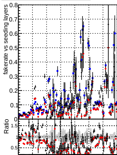
Fake rate vs. DOMstep3 ZToFF CKF DOMstep3 ZToFF default NEWT
