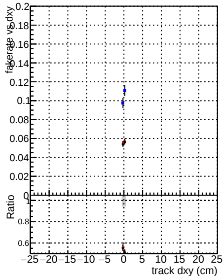
Fake rate vs d DOMstep3 TT CKF default ckPixelLess
