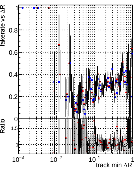
Fake rate vs \Delta R (track, jet) DOMstep3 TT CKF DOMstep3 TT default DOMstep3 TT ckfPixelLess
