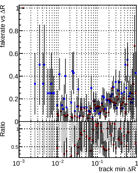
Fake rate vs \Delta R(\text{track, jet}) DOMstep3 TT CKF DOMstep3 TT default DOMstep3 TT ckfPixelLess
