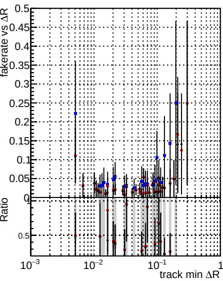
Fake rate vs \Delta R(\text{track}, \text{jet}) Legend: DOMstep3 TT CKF (blue dots) DOMstep3 TT default (red dots) DOMstep3 TT ckfPixelLess (black dots)
