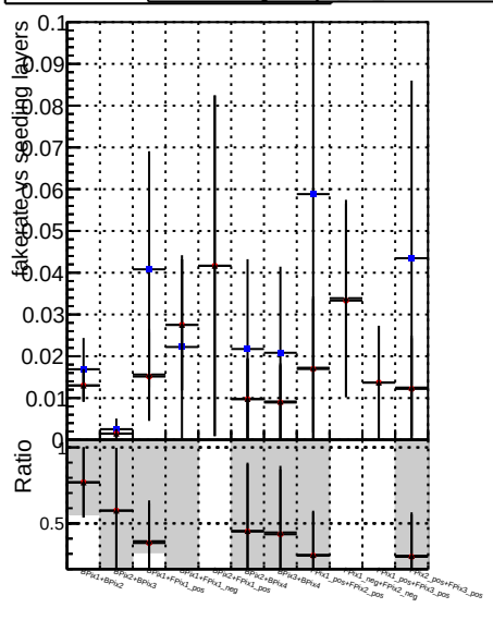
Fake rate vs. DOMstep3 CKF default
