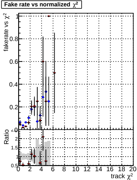
Fake rate vs. \chi^2 Legend: DOMstep3 CKF default CKFPixelLess
