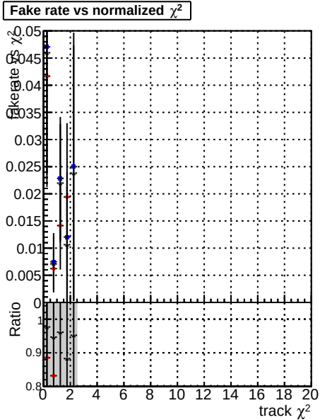
Fake rate vs. Legend: DOMstep3 TT CKF DOMstep3 default DOMstep3 CKFPixelLess
