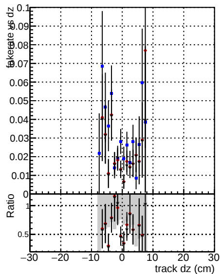
Legend DOMstep3 TT CKF default ckPixelLess Fake rate vs d Blue dots Red dots Black dots Gray dots Duplicates Rate vs Dxy Blue dots Red dots Black dots Gray dots Pileup rate vs dxy Blue dots Red dots Black dots Gray dots
