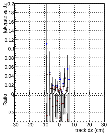
Fake rate vs dz —●— DOMstep3 TT CKF —●— default —●— DOMstep3 TT CKFPixelLess
